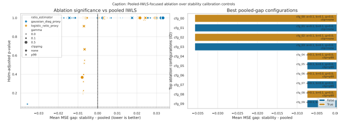
Figure 3: Pooled-IWLS-focused ablation over stability controls. Left: pooled gap (stability minus pooled) versus Holm-adjusted p-value for each ablation configuration, with dashed lines at zero gap and p = 0.05 . Right: top-ranked configurations by pooled gap. The selected configuration uses \alpha = 0.1 , \beta = 0.1 , \gamma = 0 , Gaussian ratio proxy, no clipping, and adaptive- \gamma enabled.
